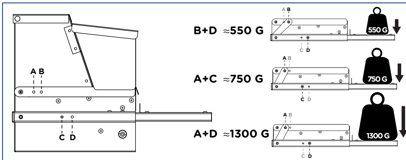
Three weight support settings
