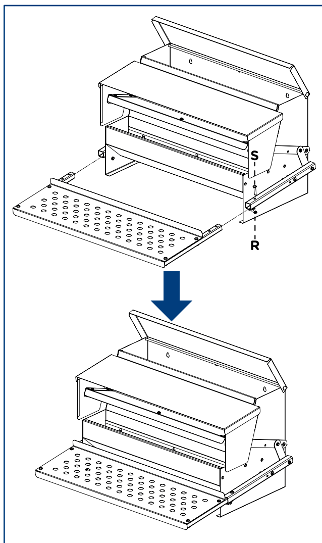
Foot pedal adjustment and insertion
