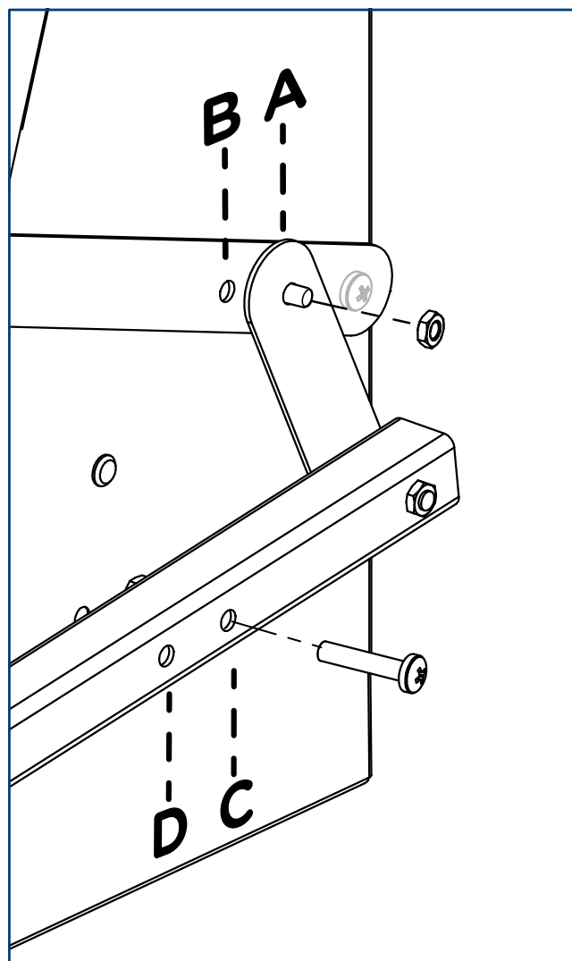
Manual adjustment for weight regulation
