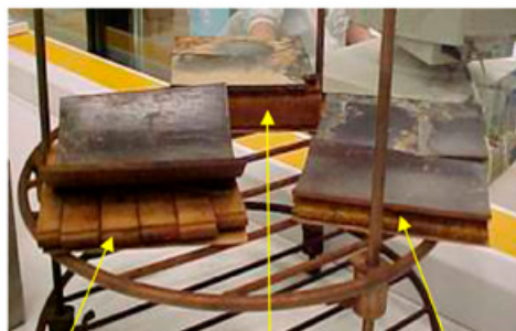
Wood core decking Hydrophobic MDF core decking Coretech
